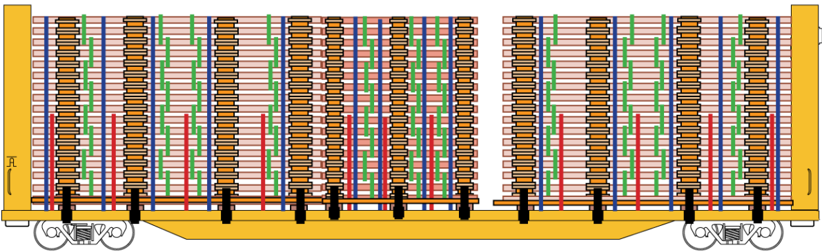
SKETCH 2: 3 PILES LOAD
