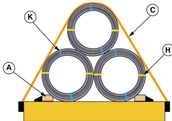
END VIEW
