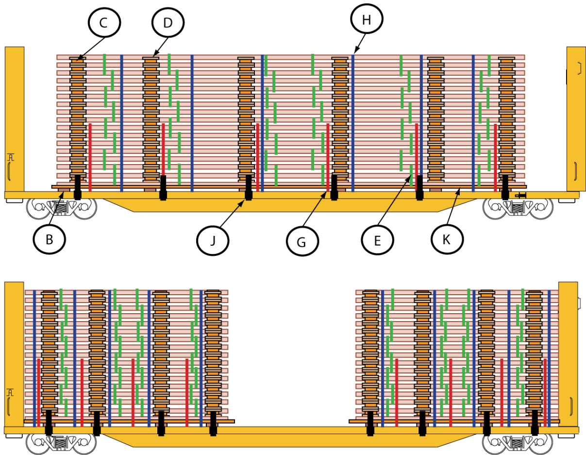
SKETCH 1: 2 PILES LOAD
